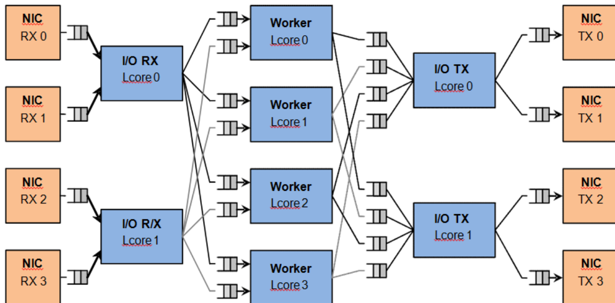
Fig. 7.10: Load Balancer Application Architecture
