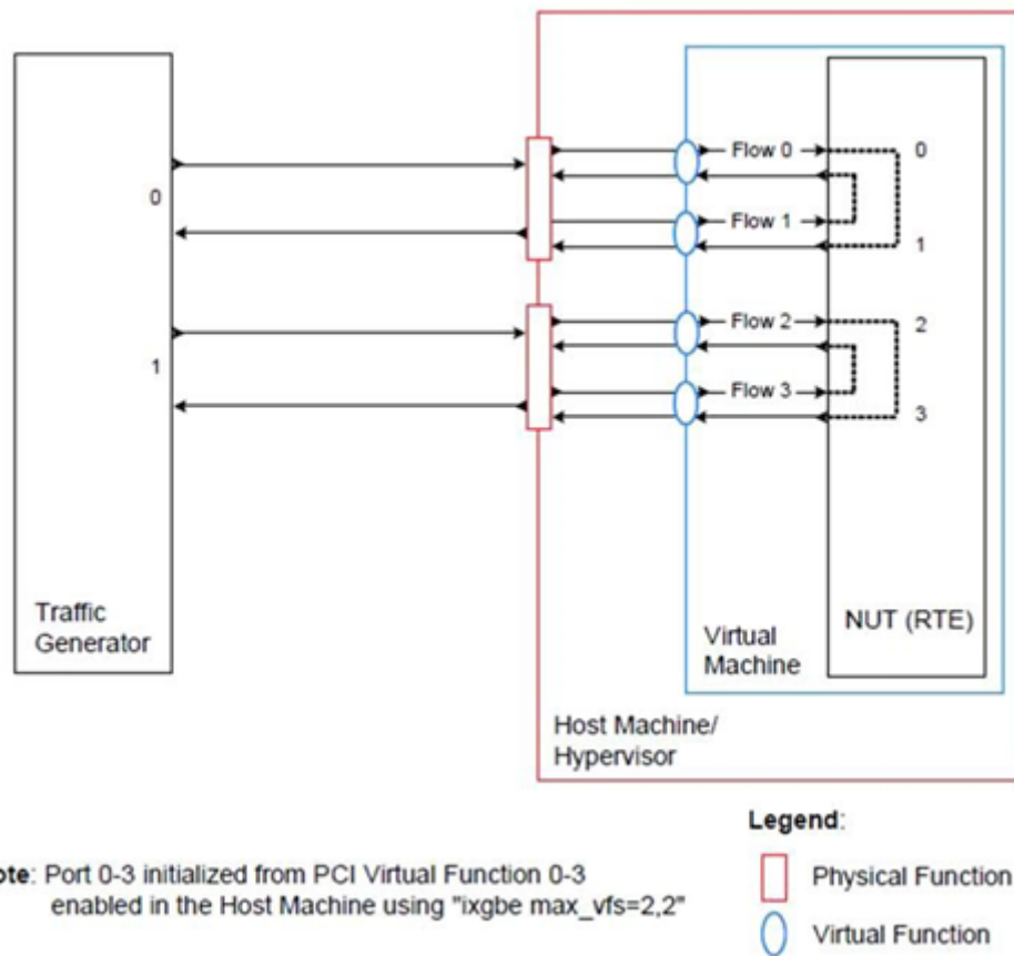
Fig. 7.7: Performance Benchmark Setup (Virtualized Environment)
