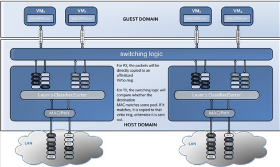
Fig. 3.1: Functionality of the DPKD Xen Packet Switching Solution.
