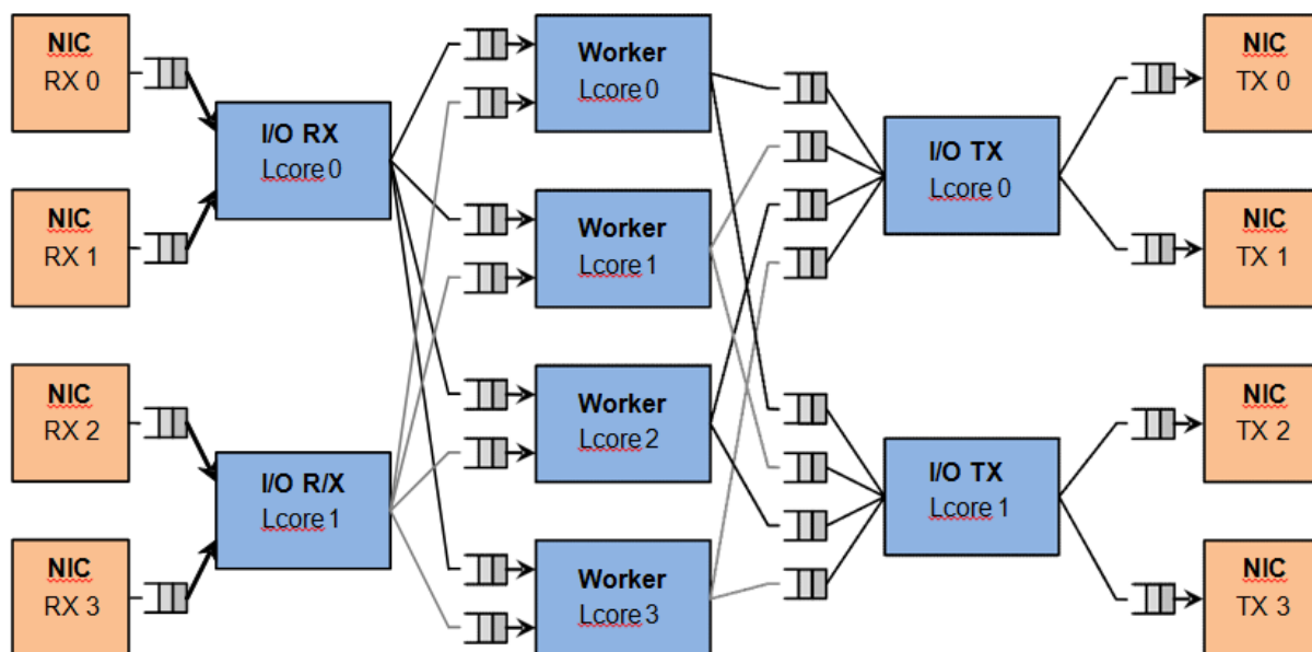
Fig. 7.10: Load Balancer Application Architecture
