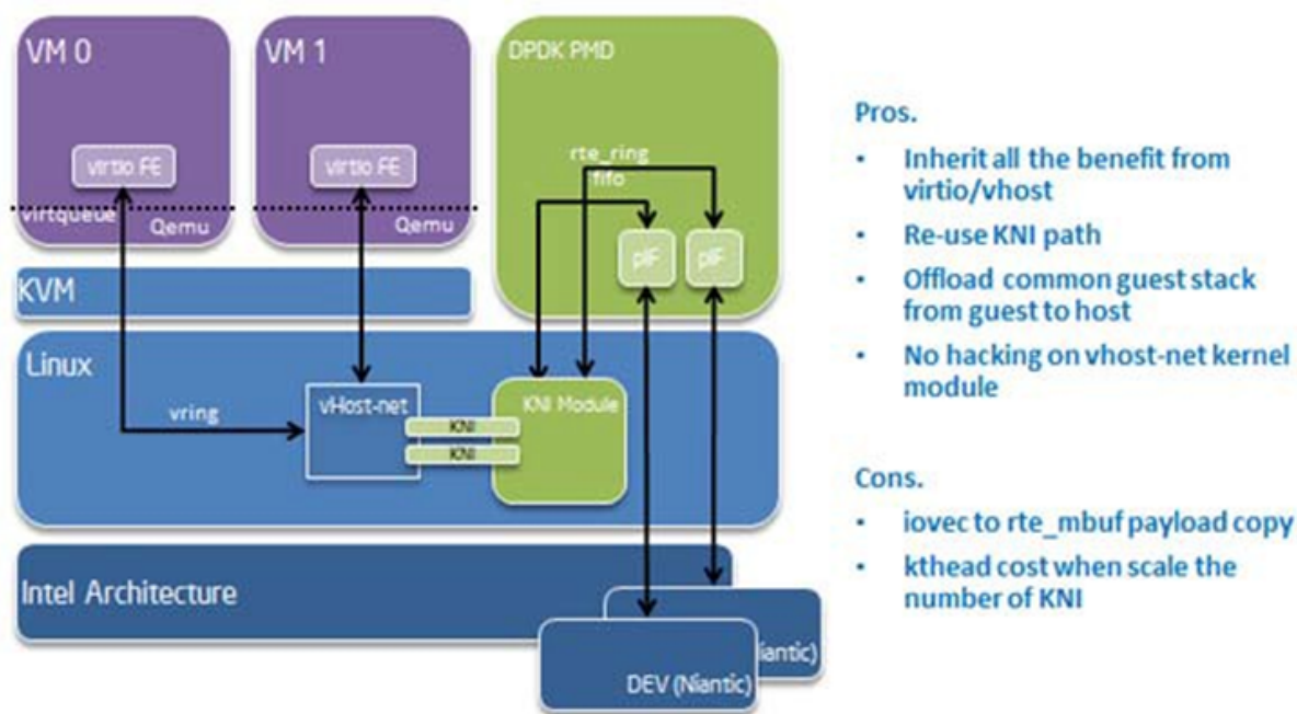
Fig. 4.38: vHost-net Architecture Overview
