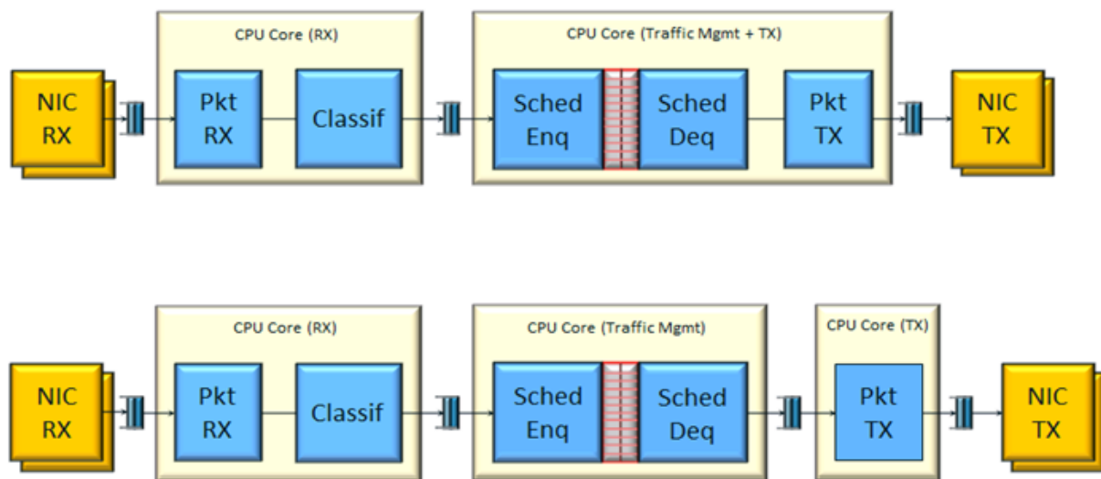
Fig. 7.15: QoS Scheduler Application Architecture
