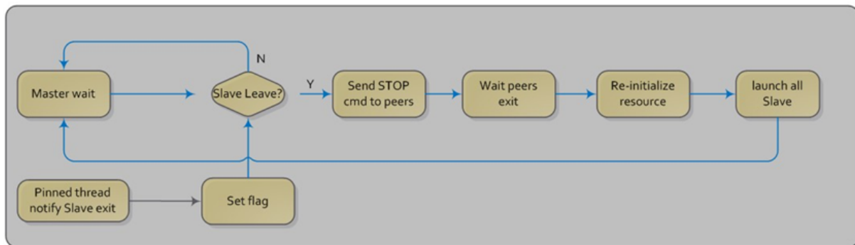
Fig. 7.14: Slave Process Recovery Process Flow
