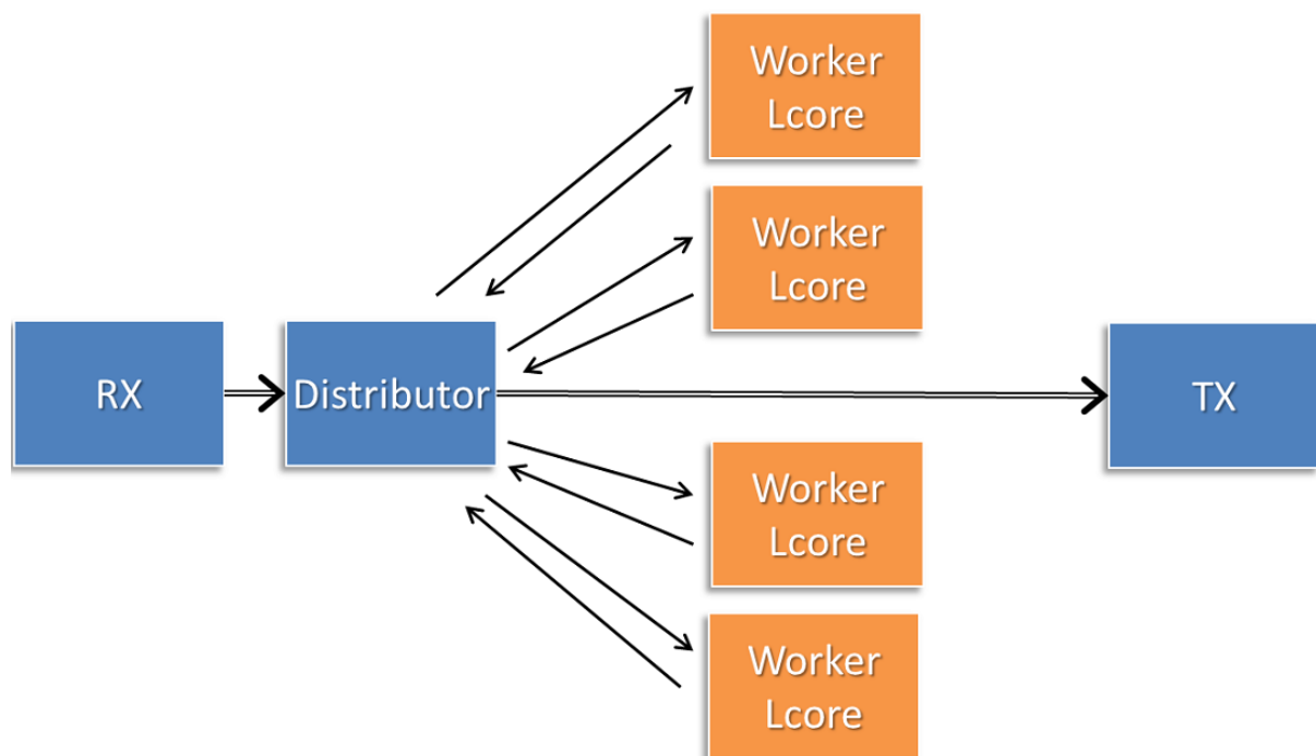
Fig. 4.34: Application workflow
