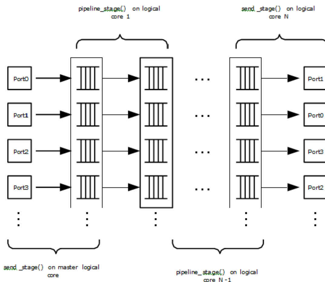
Fig. 7.19: Threads and Pipelines
