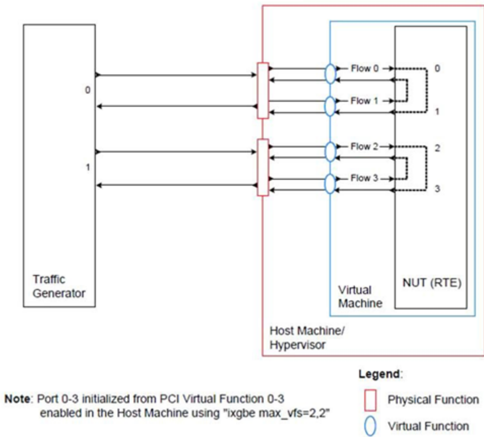
Fig. 7.5: Performance Benchmark Setup (Virtualized Environment)
