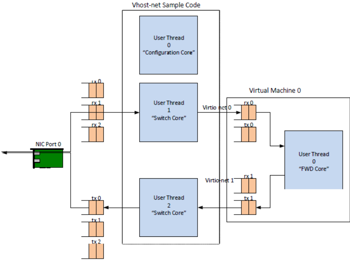
Fig. 7.24: Packet Flow Through the vhost-net Sample Application
