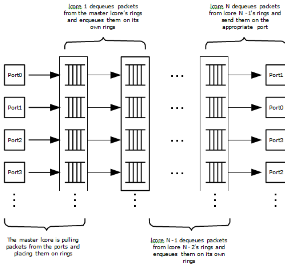
Fig. 7.17: Pipeline Overview
