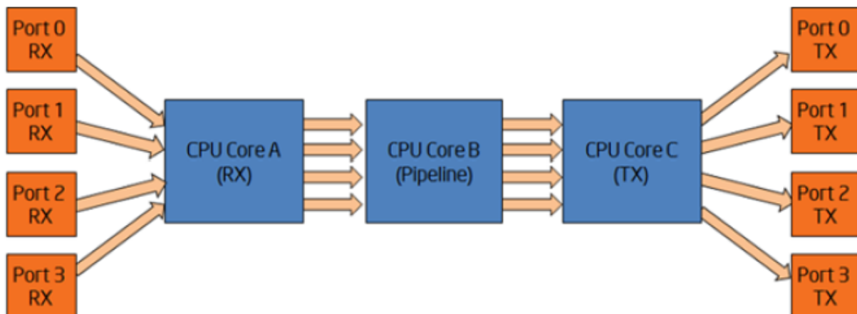
Fig. 7.29: Test Pipeline Application
