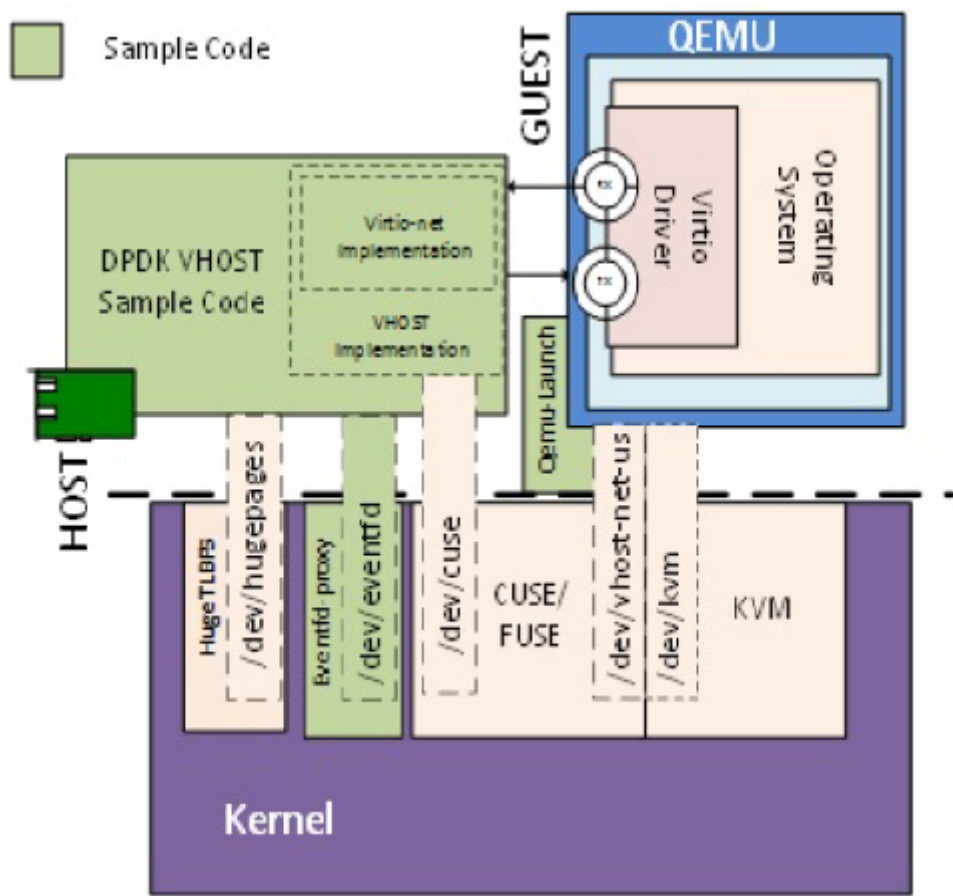
Fig. 7.23: Vhost-net Architectural Overview
