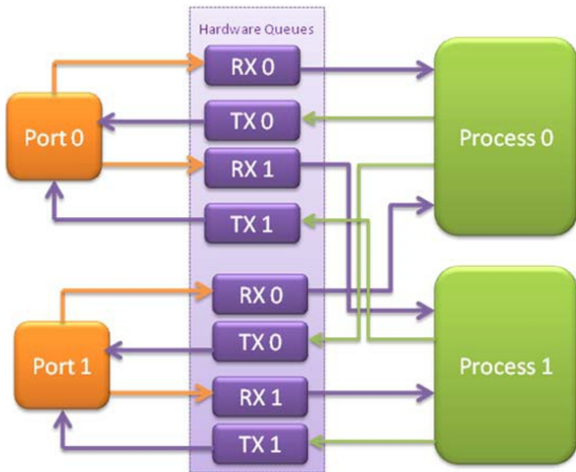
Fig. 7.11: Example Data Flow in a Symmetric Multi-process Application
