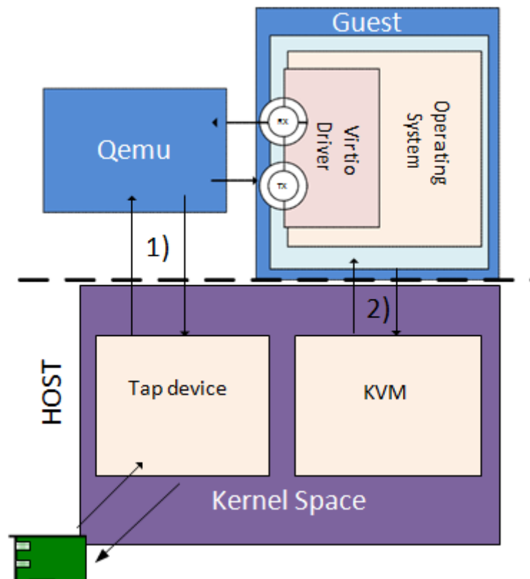
Fig. 7.21: System Architecture for Virtio-based Networking (virtio-net).
