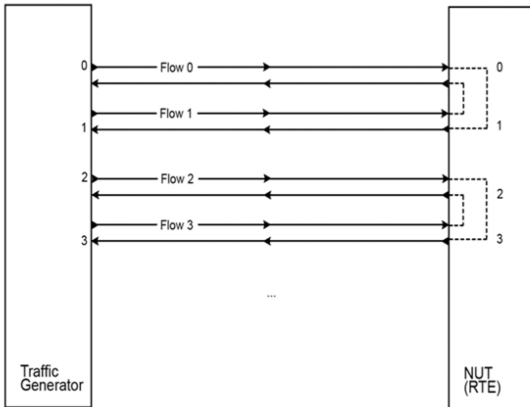
Fig. 7.18: Ring-based Processing Pipeline Performance Setup
