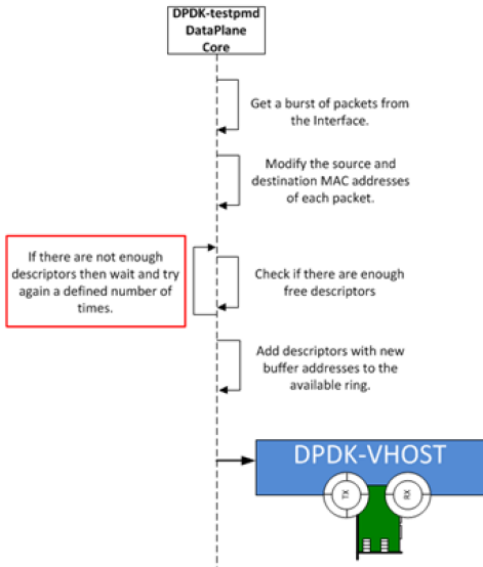
Fig. 7.25: Packet Flow on TX in DPDK-testpmd
